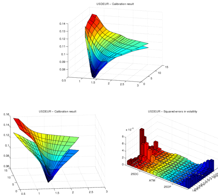
Figure 9.5: We consider a joint calibration of the implied volatility surface of USDEUR and of the two yield curves of USD and EUR simultaneously. The figure on the top compares the implied volatility surface to observed market data. As the fit is very good and the two surfaces are almost indistinguishable, on the bottom left figure we shift upwards the model implied volatility by multiplying each point by 1.1 so as to increase readability. On the bottom right we report squared errors in implied volatility for each point of the surface.
