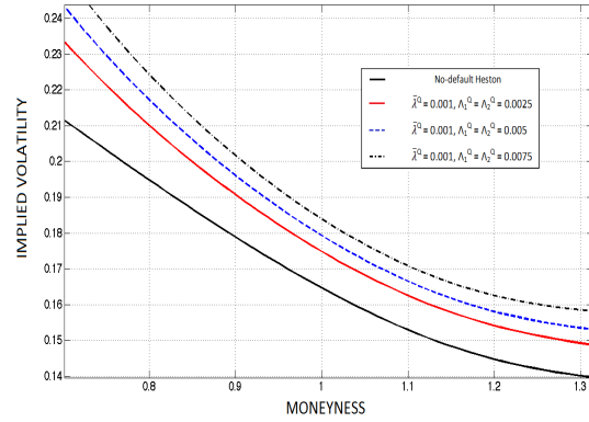
Figure 4: Implied volatility skew for different Q -intensities (for T = 1.75 ).
