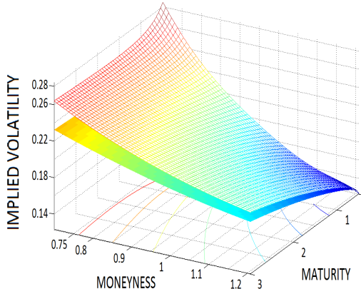
Figure 3: Implied volatility surfaces: standard Heston (solid) and Heston + Jump-to-Default (mesh).
