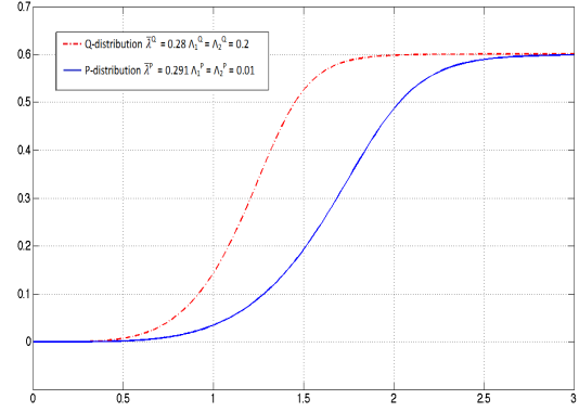
Figure 2: Distribution functions under physical ( P ) and risk-neutral ( Q ) probability measures.
